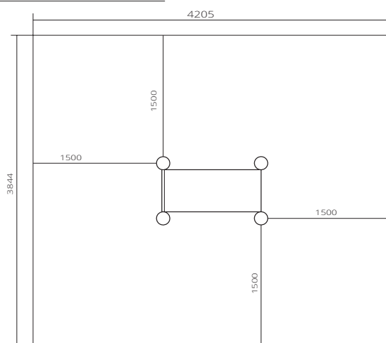
Detail benchplate
